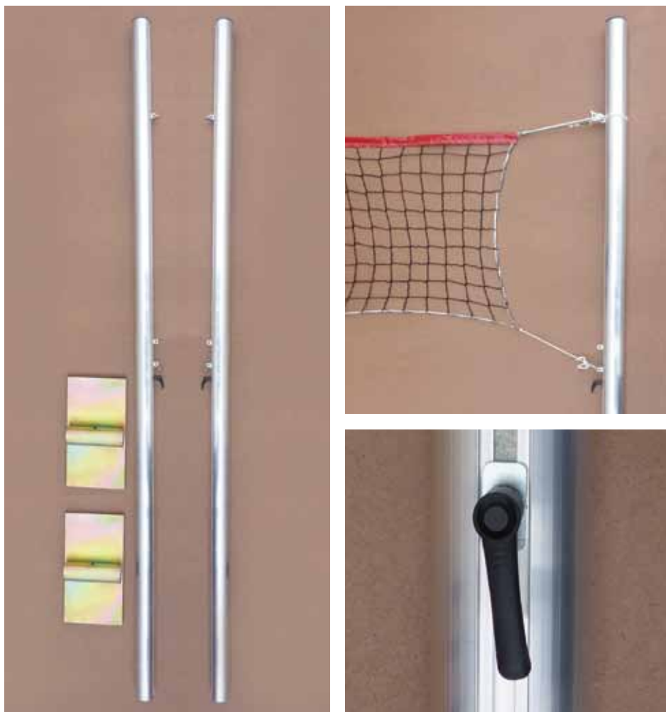
art. 5513 Impianto beach volley in alluminio, tubo \varnothing 80 mm, senza bussole Aluminium beach volley system, tube \varnothing 80 mm, without sockets
